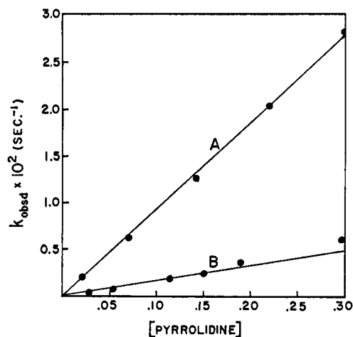
Figure 4. Plot of k_{\text{obsd}} vs. [\text{pyrrolidine}] for the reaction of cis -chalcone with pyrrolidine at 25.0° in acetonitrile (A) and heptane (B).
