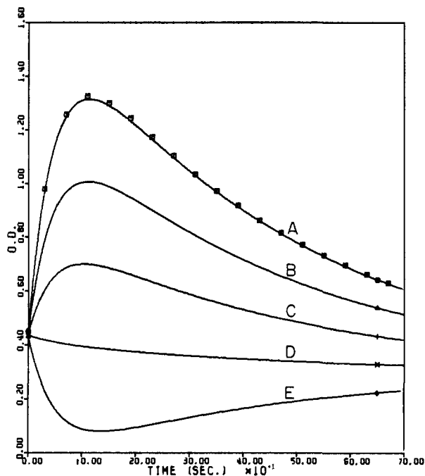
Figure 6. Computer plots of absorbance vs. time calculated from eq 10 for [pyrrolidine] = 0.244 M and \delta = 1.00 (A), 0.75 (B), 0.50 (C), 0.25 (D), and 0.00 (E). The points ( \square ) are experimental data for [pyrrolidine] = 0.244 M . \lambda = 306 \text{ m}\mu .
