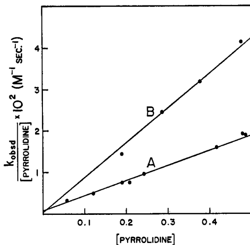
Figure 3. Plot of k_{\text{obsd}}/[\text{pyrrolidine}] vs. [\text{pyrrolidine}] for the reaction of trans -chalcone with pyrrolidine at 25.0° in acetonitrile (A) and heptane (B).
