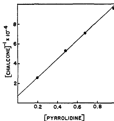
Figure 2. The data in this plot were obtained by adding trans -chalcone to several acetonitrile solutions of pyrrolidine, allowing Michael addition to proceed to equilibrium, and then determining the equilibrium chalcone concentrations. The equilibrium constant for Michael addition is derived from the slope of this plot (eq 2); C_0 = 1.87 \times 10^{-4} M .
