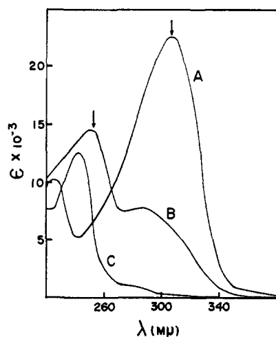
Figure 1. The spectra of trans -chalcone (A), cis -chalcone (B), and Michael adduct (C) in acetonitrile. The arrows indicate the two wavelengths used to follow the reactions in this solvent.
