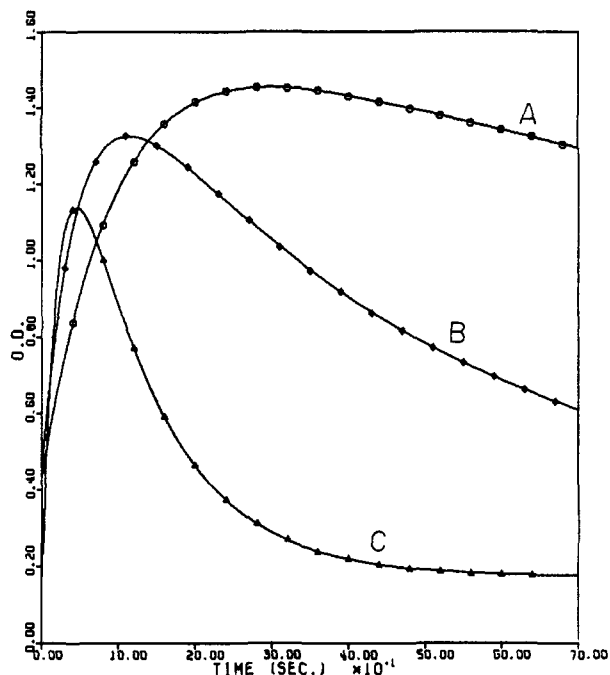
Figure 5. Computer plots of optical density vs. time for the reaction of cis -chalcone with pyrrolidine in acetonitrile at 25.0° followed at the absorbance maximum of trans -chalcone (306 m \mu ). The solid curves are theoretical lines calculated from eq 10; the points are experimental. The pyrrolidine concentrations are 0.122 M (A), 0.244 M (B), and 0.487 M (C). Excellent agreement between experiment and theory was also found at two higher concentrations of amine, but the curves are omitted to avoid cluttering.
